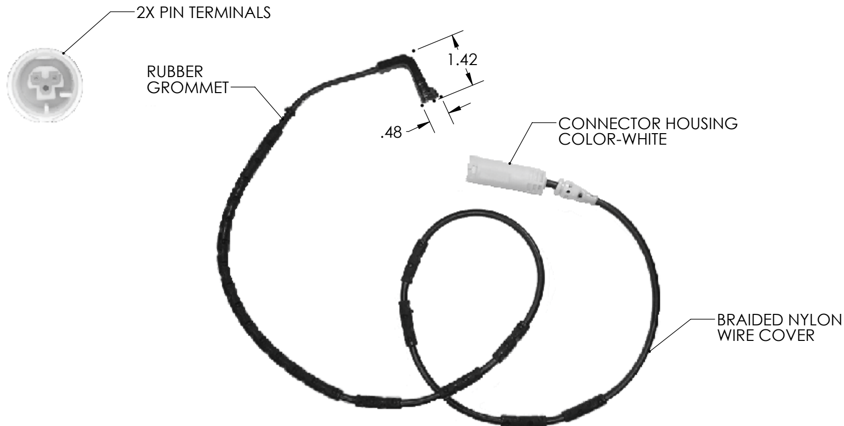
BRAKE PAD WEAR SENSOR ASSEMBLY(42.75) INCLUDING CONNECTOR TO CENTER LINE OF SENSOR
