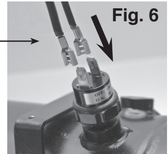
The compressor's (-) negative wire and the wire provided with the loop terminal are both connected to the pressure switch terminals. There is no polarity, so either wire can be connected to either pressure switch terminal.
