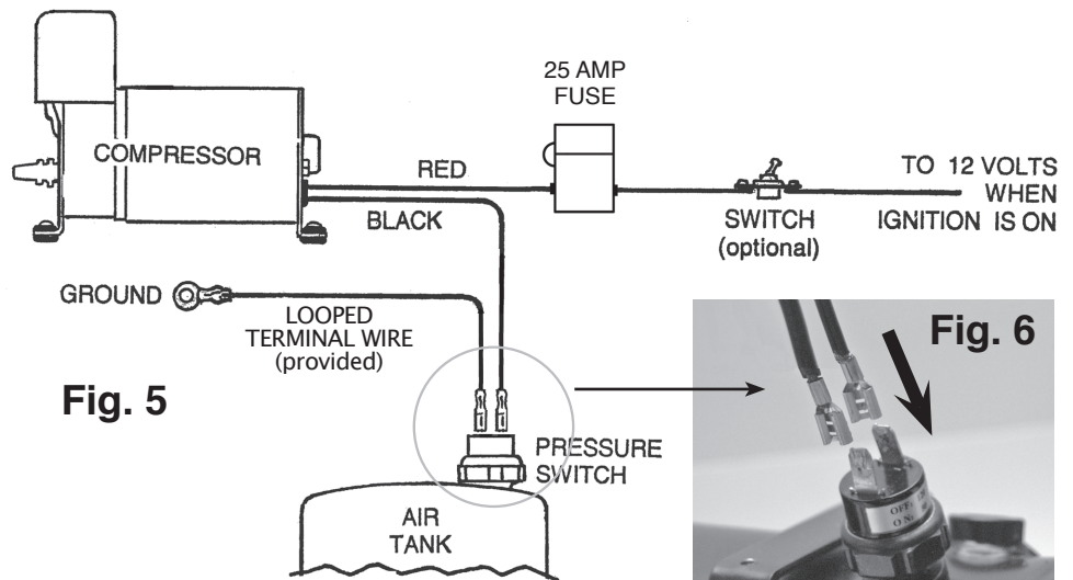
The compressor's (-) negative wire and the wire provided with the loop terminal are both connected to the pressure switch terminals. There is no polarity, so either wire can be connected to either pressure switch terminal.
