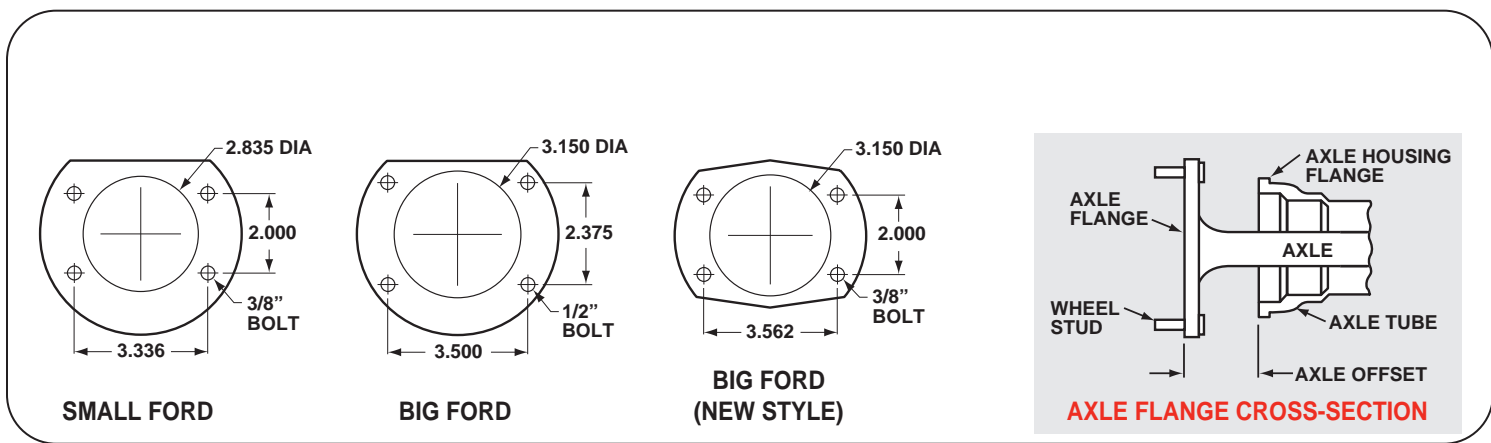
Bronco Housing Flange / Axle Offset
