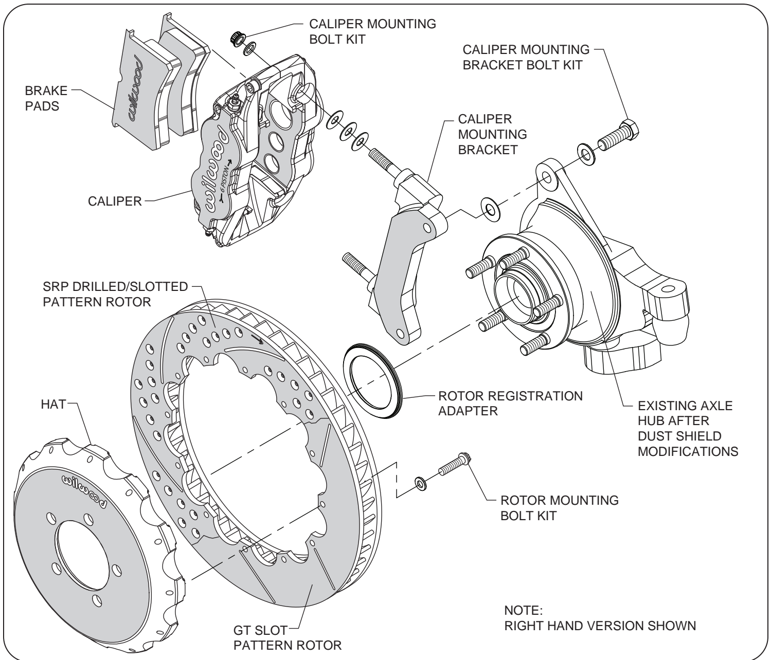
Typical Installation Diagram (FNSL6R 13.06" Kit Shown)
