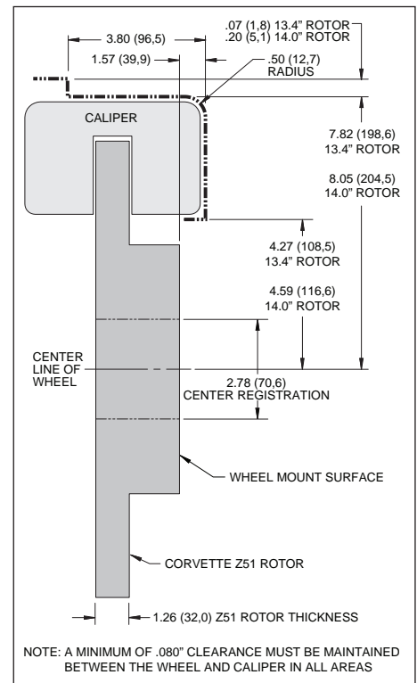
Wheel Clearance Diagram
