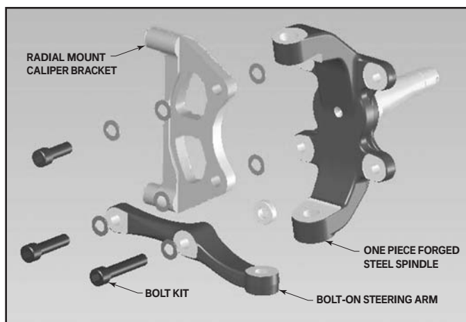
Typical View of Radial Bracket Installation
