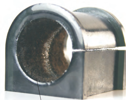
PTFE LINING
