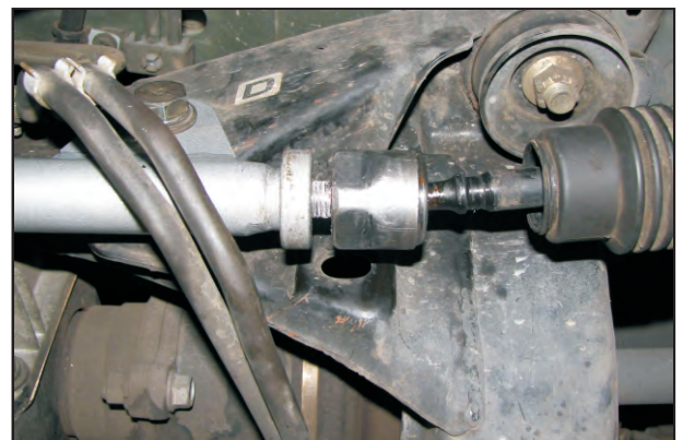
Photo 2: Inner tie-rod fitment
