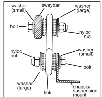
Figure 2. Link assembly guide.
