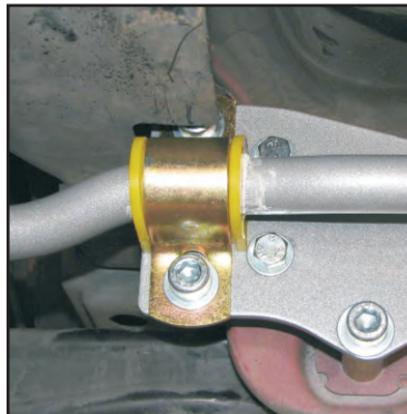
Photo 2. Swaybar mounting.
