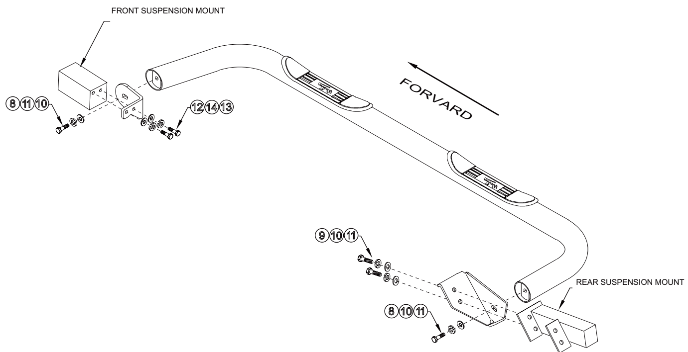
INSTALLATION VIEW OF PASSENGER SIDE SHOWN, DRIVER SIDE OPPOSITE
