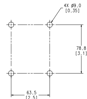
Mounting Bolt Pattern
