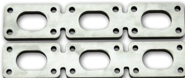
Part No. 14636
