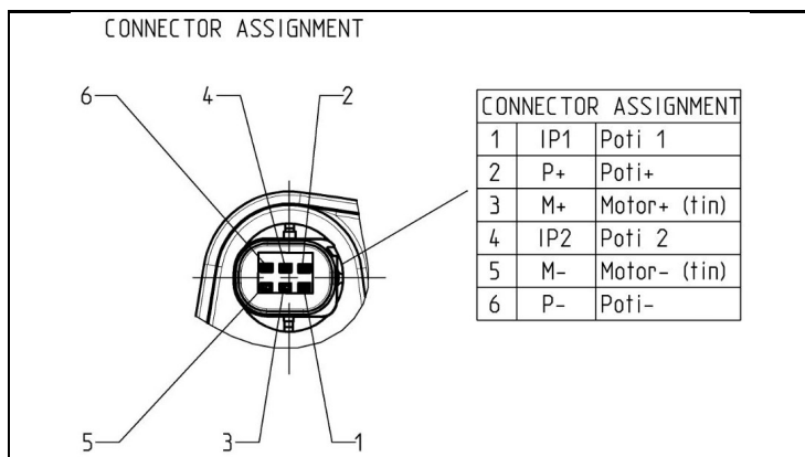
2 - Connector
