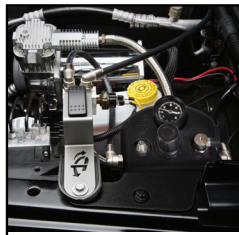
Part # 269-0717 GEN 2 Jeep Jk 4 Tire Inflation System On Board ADS Rear Engine Controller Box
