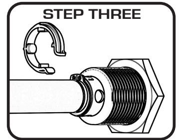
REMOVE PLASTIC CLIP BY PUSHING ON TABS. DISCARD CLIP.
