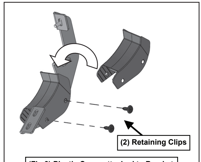
(Fig 8) Plastic Cover attached to Bracket
