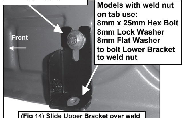
(Fig 14) Slide Upper Bracket over weld nut if equipped-also see Figure 2
