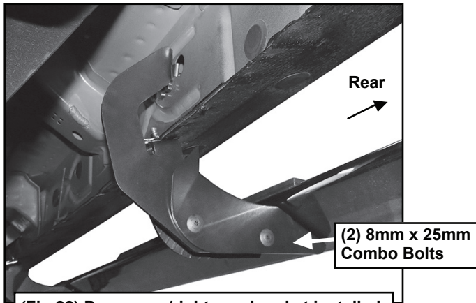
(Fig 22) Passenger/right rear bracket installed
