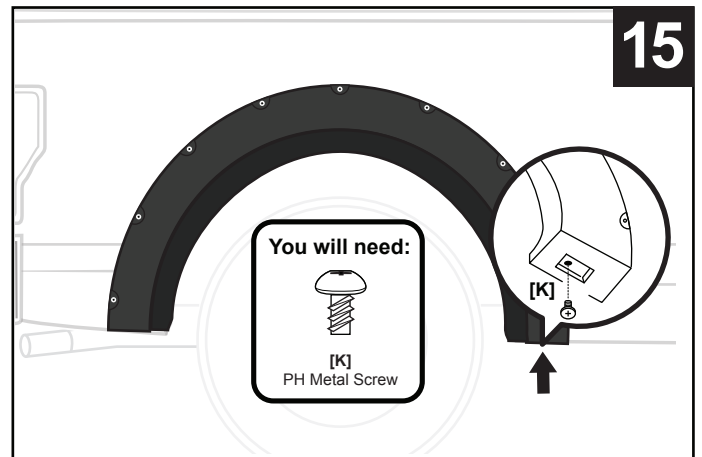
15. Install supplied PH Metal Screw [K] through lower flare hole into the S-Clip.
