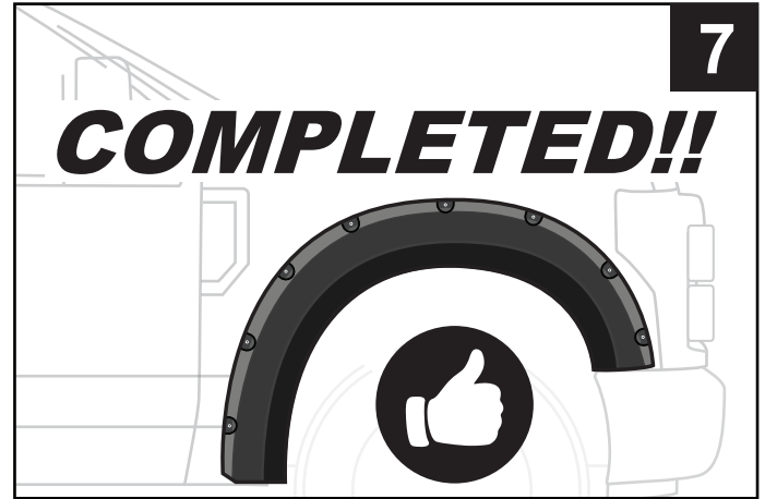
7. Tighten all 5 screws from STEPS 5-6 to complete. Repeat STEPS 1-7 for driver side front flare.
