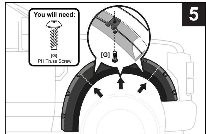
5. Tightly press flare against vehicle to evenly remove space between flare and vehicle by aligning 3 top flare holes to inner bracket clip holes. Then install 3 PH Screws [G] through flare holes into clip holes without tightening
