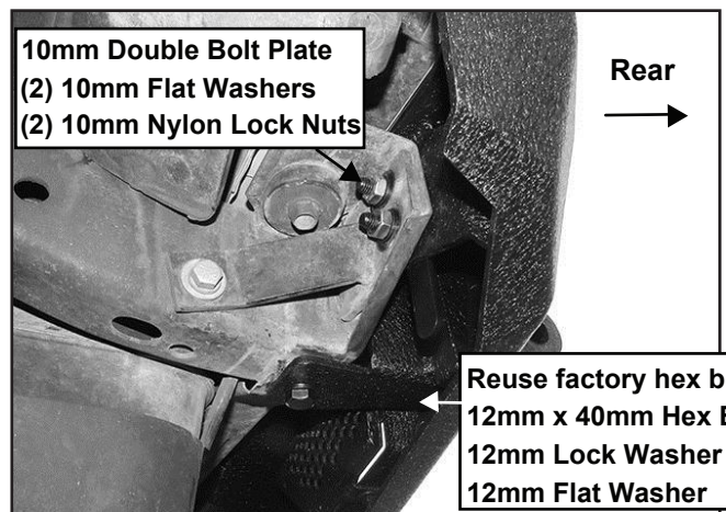
(Fig 6) Bumper installed (driver/left side pictured from below)
