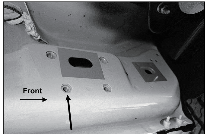
(Fig 8) Driver/left side front mid 2015-on (example of models with factory installed threaded inserts)
