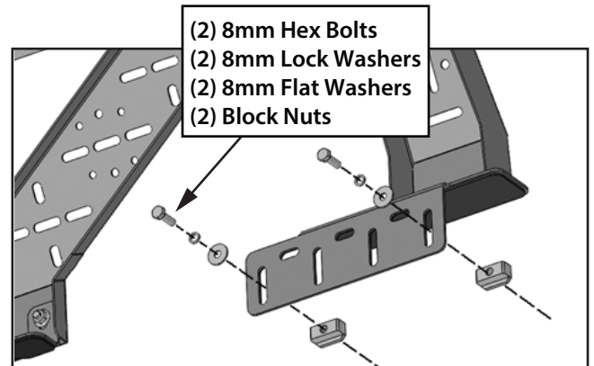
(Fig 15) Attach the Overland Bed Rack assembly to the Block Nuts
