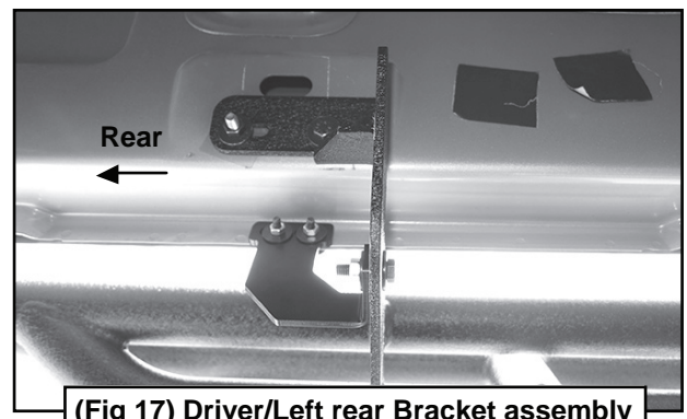
(Fig 17) Driver/Left rear Bracket assembly
