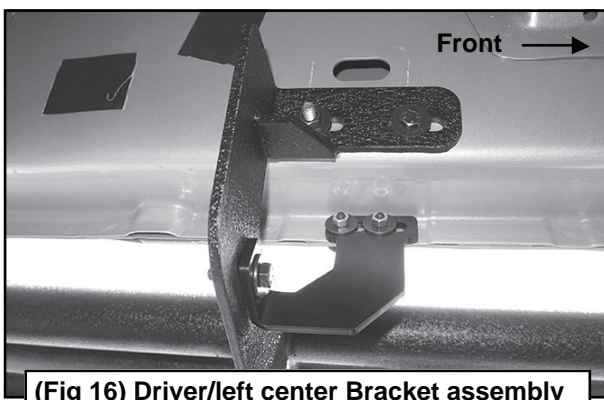
(Fig 16) Driver/left center Bracket assembly
