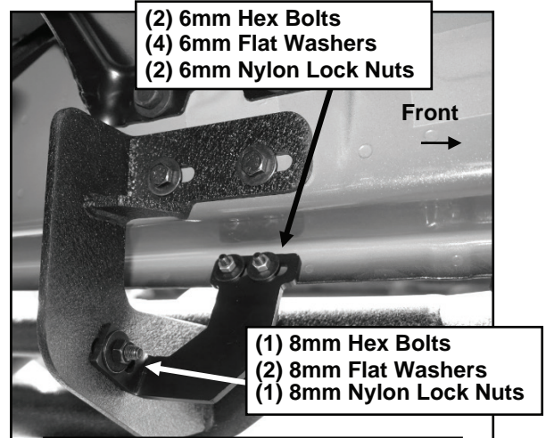
(Fig 10) Driver side front bracket
