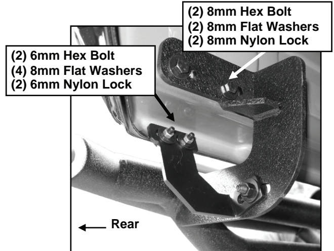
(Fig 14) Driver/Left rear Mounting Bracket assembly
