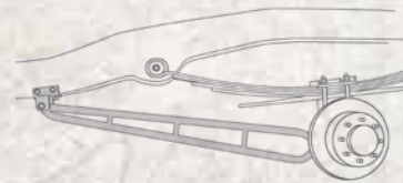
Ladder Bars
