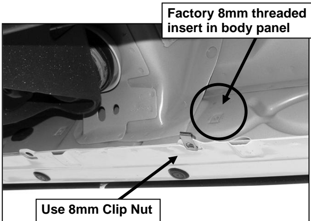
(Fig 1) Driver side (2) mounting locations
