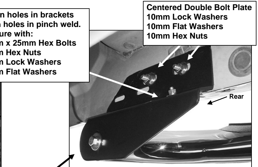
(Fig 4) Rear Mounting Bracket installation
