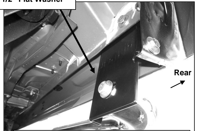
(Fig 7) Passenger Side Rear Bracket Inside View
