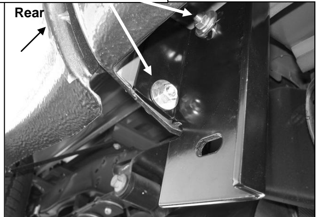
(Fig 5) Passenger Side Rear Bracket Outside View
