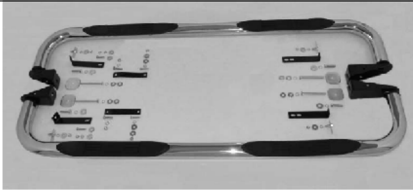
FULL ASSEMBLY -
