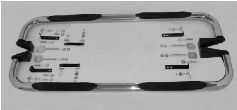
FULL ASSEMBLY -
