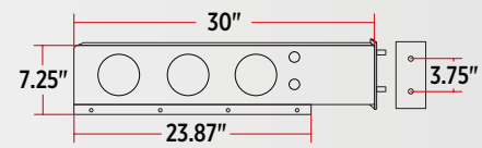
RED STOP, TURN & TAIL TO PURPLE AUXILIARY TU-9209L5 Clear Lens
