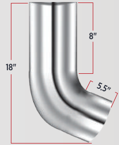
5" DIAMETER TEL55-PET
