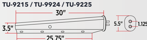
▲ PAINTED STEEL TU-9225
