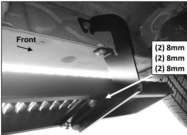
(Fig 10) Driver/left front Bracket installed
