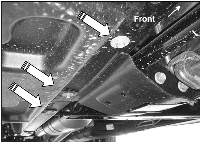
(Fig 12) 07-16 Passenger side front pictured with DEF tank cover. Remove (3) hex bolts to remove cover
