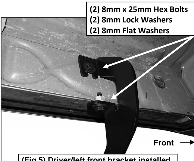
(Fig 5) Driver/left front bracket installed
