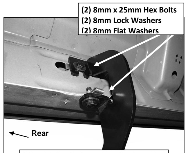
(Fig 6) Driver/left rear bracket installed
