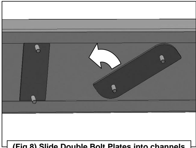
(Fig 8) Slide Double Bolt Plates into channels
