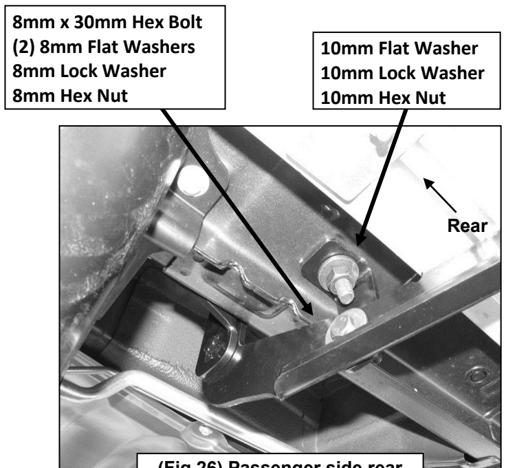
(Fig 26) Passenger side rear Bracket pictured from below
