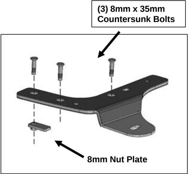
(Fig 11B) Attach Passenger/right Rear Mounting Bracket to top of body
