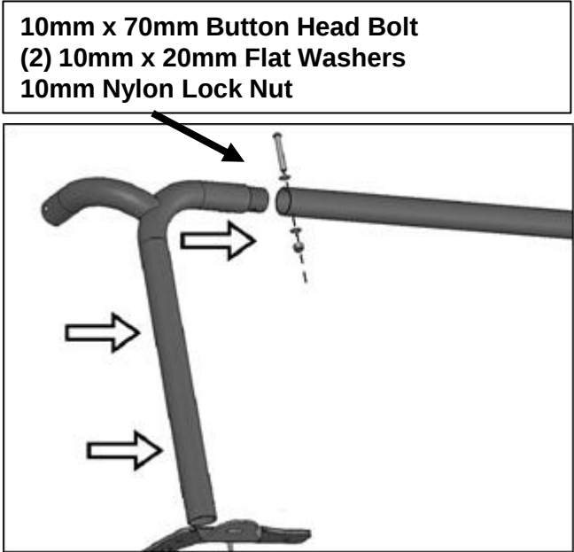
(Fig 17) Attach passenger/right Rear Leg to Sidebar
