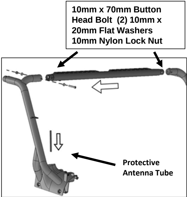
(Fig 8) Slide (1) Crossbar into the top of the installed passenger/right Front Rack Leg. Attach Crossbar to driver/left Rack Leg. NOTE: Crossbar can be installed with light tabs facing forward or to the back if desired
