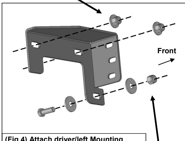
(Fig 4) Attach driver/left Mounting Bracket to end of frame
