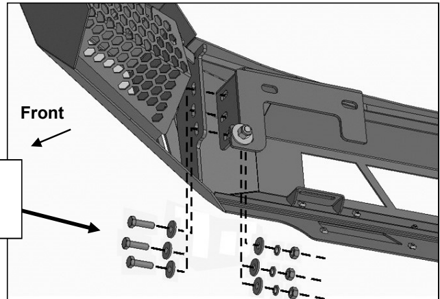
(Fig 11) Attach Bumper to Frame Mounting Bracket
