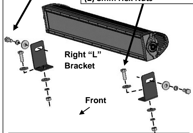
(Fig 8) Example of center light installation
