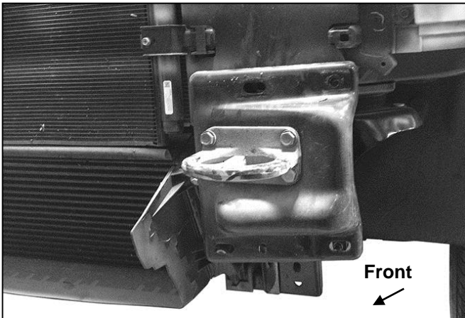
(Fig 5) Remove tow hook (Driver side pictured)
