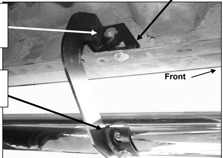
(Fig 5) Driver Side Center Mounting Bracket location
