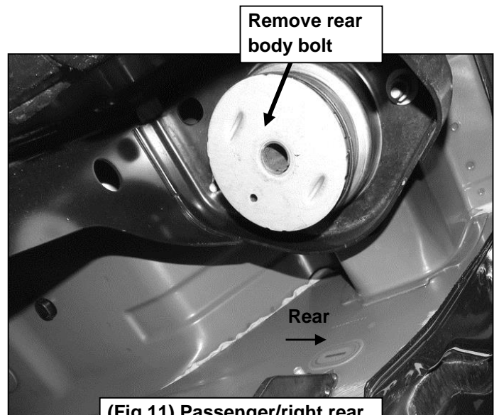
(Fig 11) Passenger/right rear body bolt mounting location
