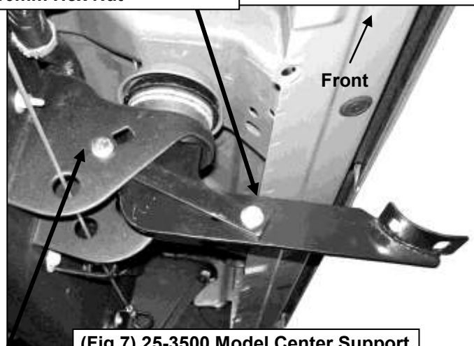
(Fig 7) 25-3500 Model Center Support Bracket Installation Pictured.
