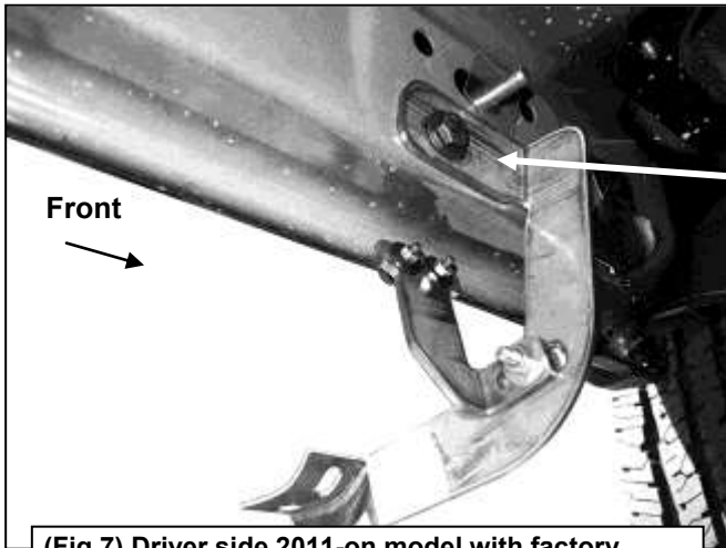
(Fig 7) Driver side 2011-on model with factory holes in pinch weld pictured. IMPORTANT: 2009-2010 models without holes in pinch weld will require drilling 1/4" holes through pinch weld to attach driver side front support bracket. Do complete installation of sidebars first, level sidebar before drilling holes for support bracket.
