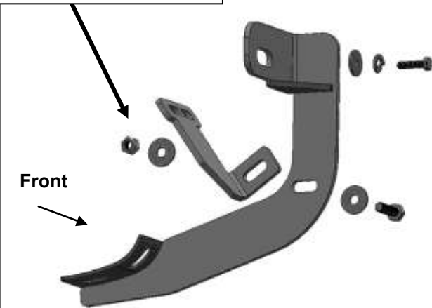
(Fig 5) Driver/Left front Mounting Bracket assembly
