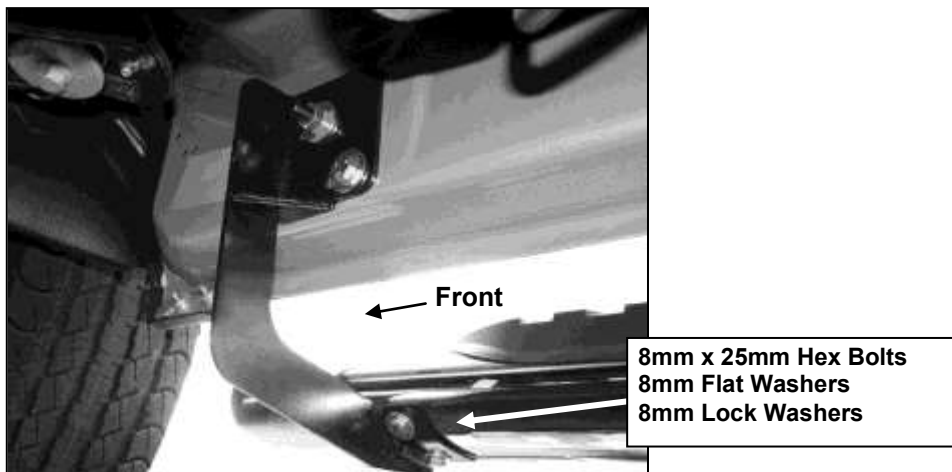
(Fig 13) Passenger/right front Mounting Bracket
