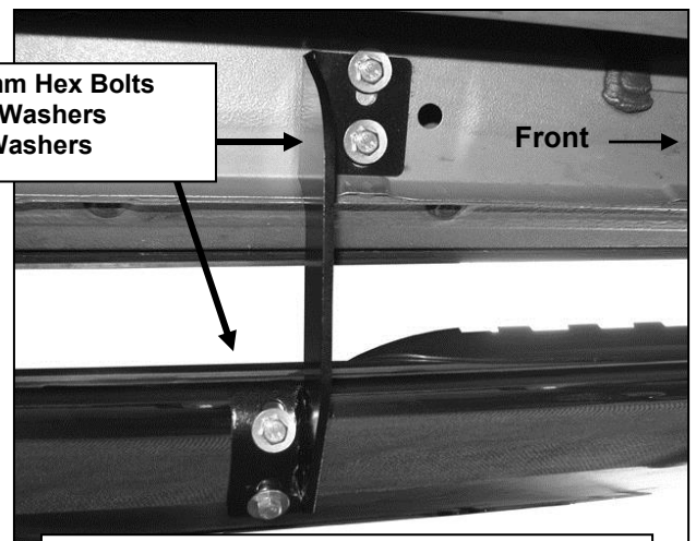
(Fig 4) Driver/Left Center Bracket Pictured
