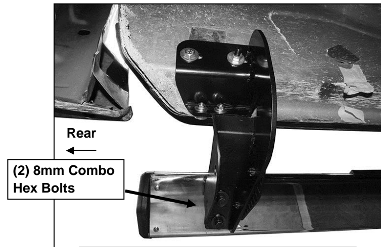
(Fig 19) Driver/left rear Bracket assembly
