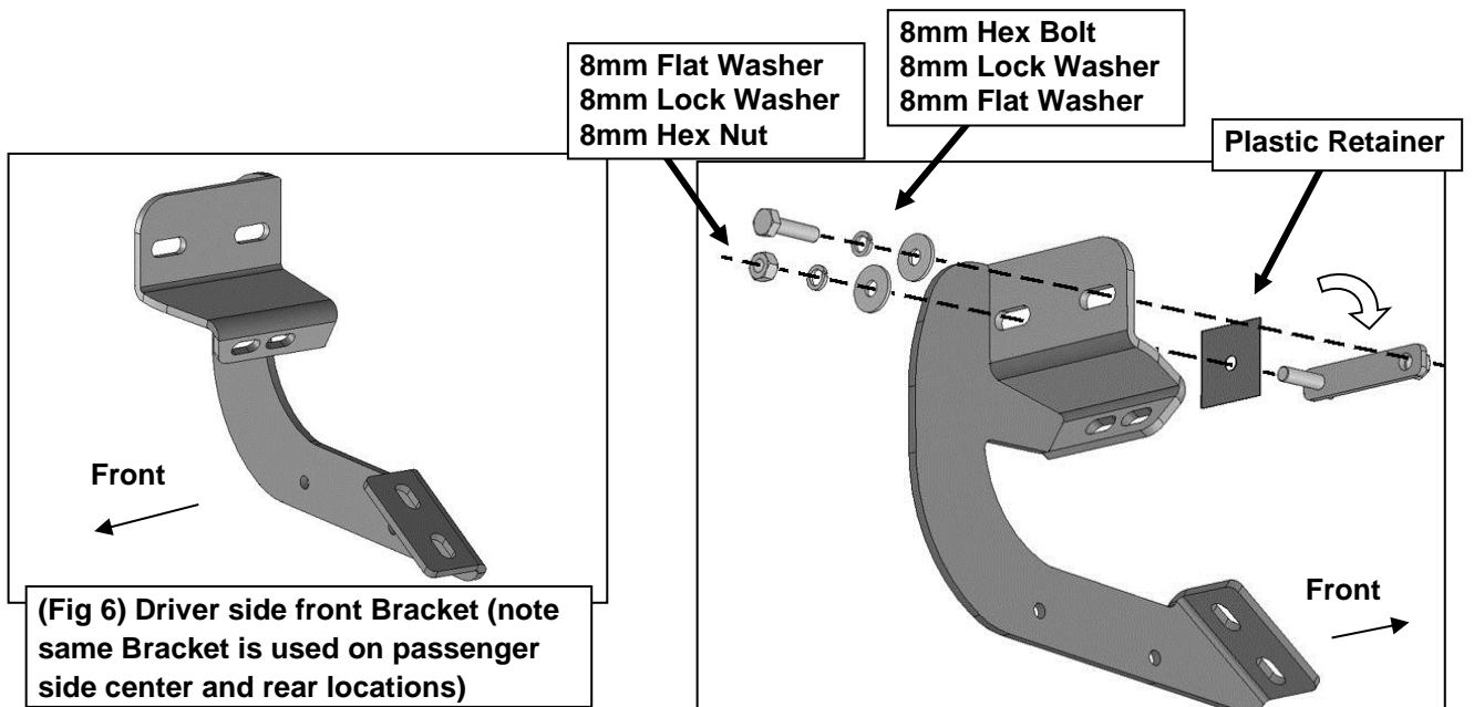
(Fig 7) Attach Bracket to threaded end of Bolt Plate first. Remove 8mm Hex Bolt (see Fig 3). Rotate Bolt Plate to line up with remaining factory hex shaped hole.
