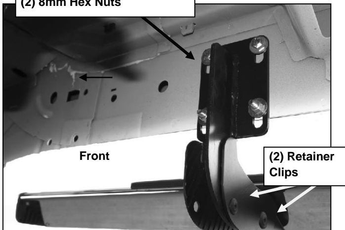
(Fig 5) Passenger/right front Bracket installation pictured
