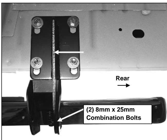
(Fig 6) Passenger/right rear Bracket pictured
