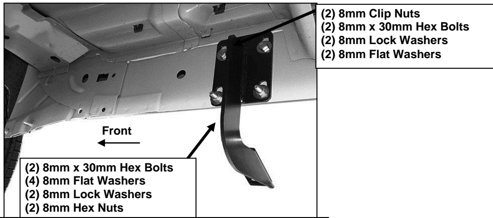
(Fig 4) Passenger/right front Bracket installation pictured
