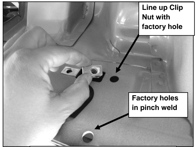
(Fig 2) Typical Mounting Location
