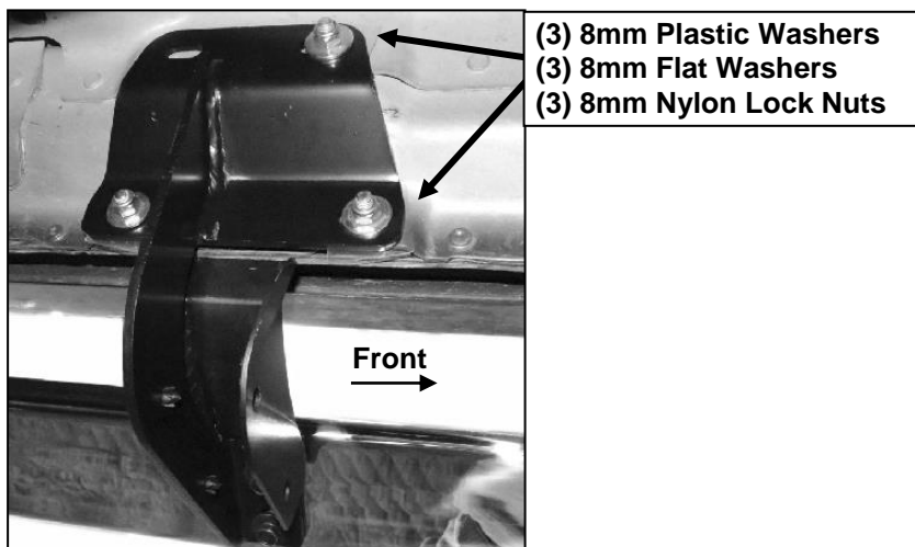
(Fig 4) Driver side front Bracket installation
