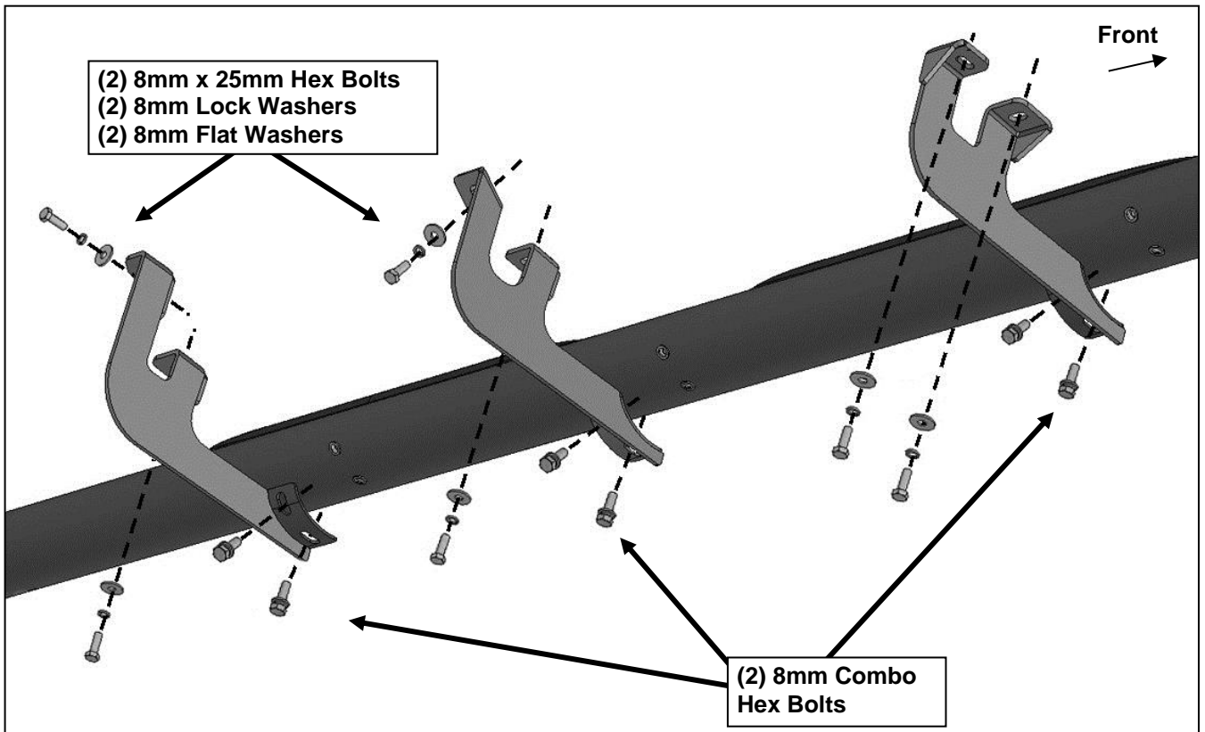
(Fig 8) Complete driver/left installation
