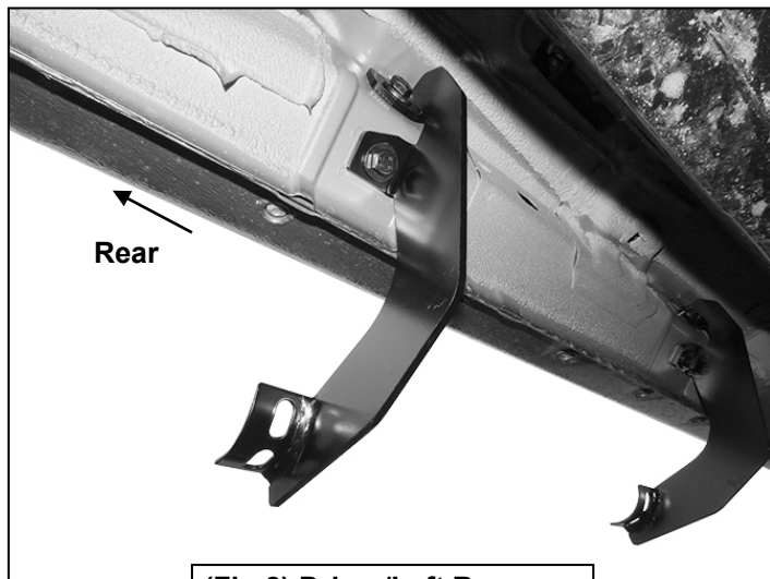
(Fig 8) Driver/Left Rear Mounting Bracket installed
