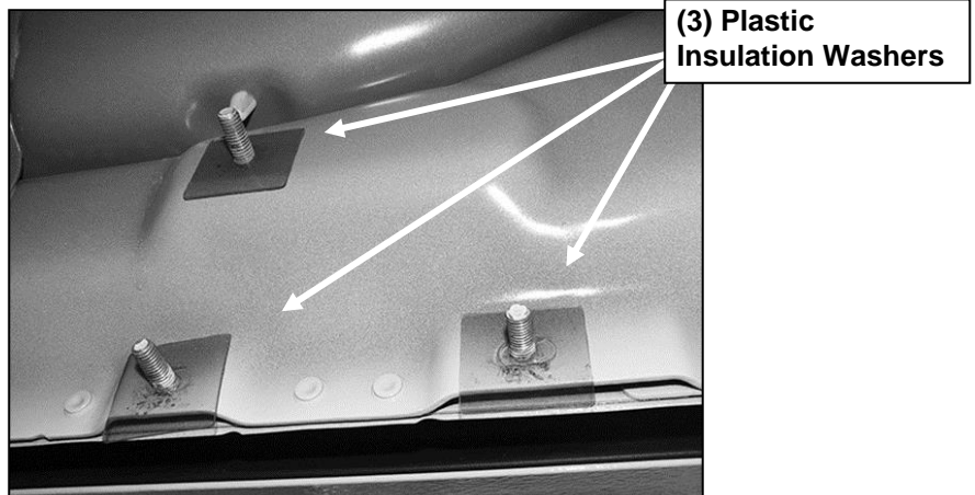
(Fig 3) Thread Plastic Washers onto all mounting studs. Passenger side rear pictured
