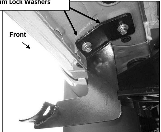
(Fig 2) Driver side front mounting location pictured
