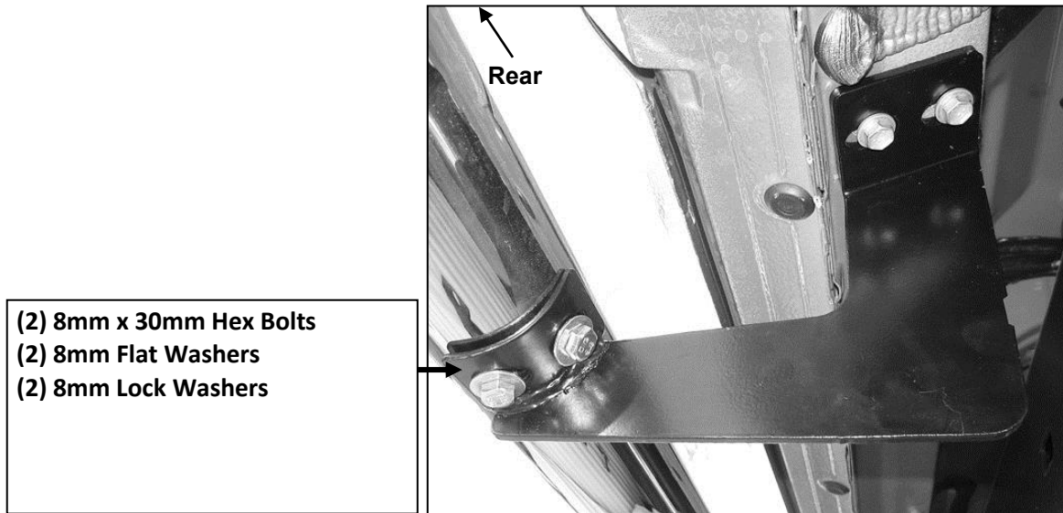
(Fig 4) Driver side rear mounting location pictured
