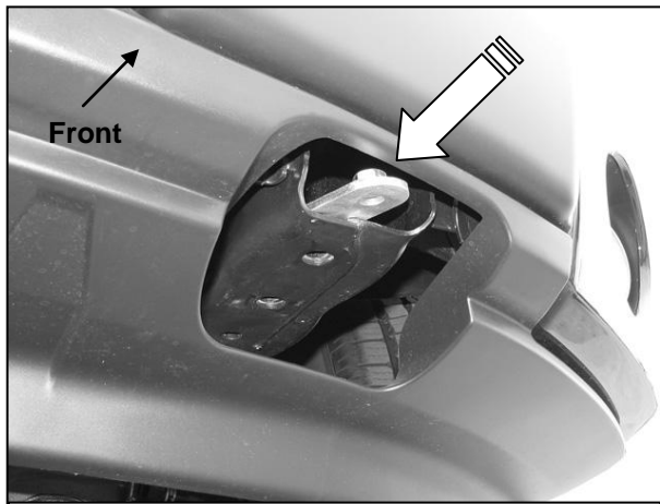
(Fig 5B) Insert Nut Plate through opening in end of frame (NOTE: Tow hook model pictured for instruction purposes only)
